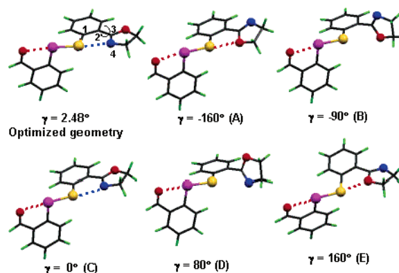
Figure 5. Variation of the relative stabilization energy of 27 for the rotation of the oxazoline ring around the C–C bond attached to the benzene ring. The calculations were performed at the B3LYP/6-31G* level of theory.
